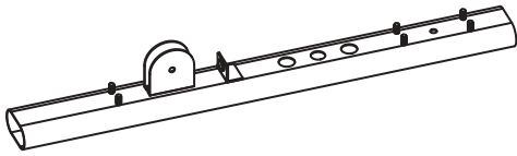
(1R) BASE FRAME LEG - RIGHT
